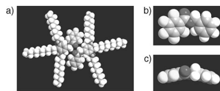
Figure 5. Molecular models for a) disk-shaped dimer of 3 ( R = n\text{-C}_{10}\text{H}_{21} ) and the most stable conformer of phenylmethyl pentafluorobenzoate shown from the front (b) and side (c) views (calculated by AM1).
